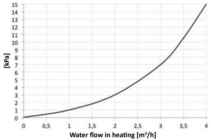
Pressure drop in the plate heat exchanger
