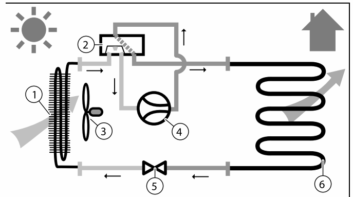
figure 1 Heating mode
