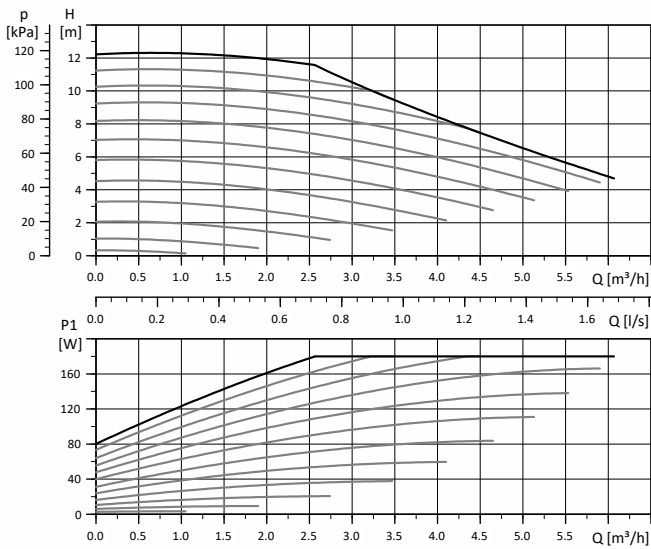
figure 1 Heating mode
