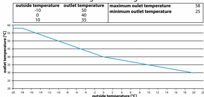
Heating curve setting
